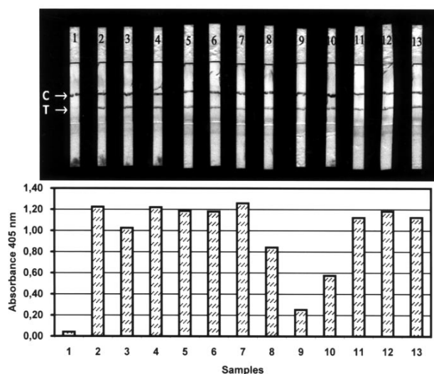
Fig. 1. Detection by lateral flow and DAS ELISA of Pepino mosaic virus in tomato. Sample 1 is healthy control, samples 2 to 8 are from leaves and samples 9 to 13 are from fruits. T indicates the test line and C indicates the control line.
