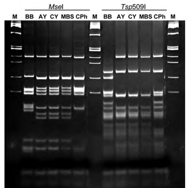
Fig. 5. RFLP analysis of nusA gene sequences amplified in polymerase chain reactions (PCRs) primed by oligonucleotide pair PhNusF2/PhNusR5 from phytoplasma strains, BB, AY (AY1), CY, MBS and CPh. Products from PCRs were digested with restriction endonucleases MseI and Tsp509I . M, \phi X174 RFI DNA HaeIII digest size standard, fragment sizes (bp) from top to bottom: 1353, 1078, 872, 603, 310, 281, 271, 234, 194, 118, 72.
