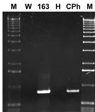
Fig. 1. Amplification of nusA gene sequences, 0.8 kbp in size, from clover phyllody (CPh) phytoplasma DNA. Polymerase chain reactions were primed by oligonucleotide pair PhNusF1/PhNusR5; annealing temperature was 55°C. W, reaction mixture devoid of template DNA. 163, template was derived from DNA clone CPh163 containing an insert that included the nusA gene. H, healthy plant ( C. roseus ) DNA template. CPh, CPh phytoplasma infected plant DNA template. M, 1 Kb DNA Ladder.
