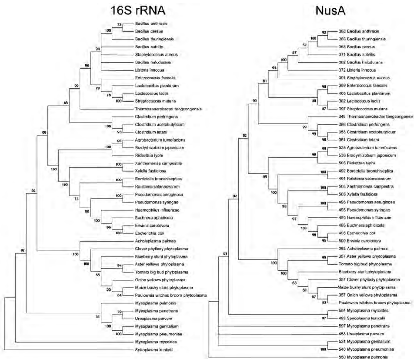
Fig. 3. Phylogenetic trees constructed by the Neighbor-Joining method of 16S rRNA gene sequences (left) and NusA amino acid sequences (right) from clover phyllody (CPh), onion yellows (OY-M), aster yellows (AY-WB), blueberry stunt (BBS3), tomato big bud (BB), paulownia witches' broom (PaWB), and maize bushy stunt (MBS) phytoplasmas; Acholeplasma palmae ; Spiroplasma kunkelii , five Mycoplasma and one Ureaplasma species, and 28 walled bacteria. Numbers indicate numbers of amino acids in full length NusA proteins where known.
