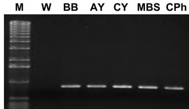
Fig. 4. Amplification of 1 Kbp nusA gene sequences from phytoplasmas belonging to group 16SrI, subgroups 16SrI-A (tomato big bud phytoplasma, BB), 16SrI-B (aster yellows, AY [AY1]; chrysanthemum yellows, CY; maize bushy stunt, MBS), and 16SrI-C (CPh, clover phyllody phytoplasma). M, 1 Kbp DNA Ladder. W, polymerase chain reaction (PCR) mixture devoid of template DNA. Polymerase chain reactions were primed by oligonucleotide pair PhNusF2/PhNusR5.
