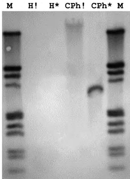
Fig. 2. Southern hybridization of the nusA gene in clover phyllody phytoplasma genome. Genomic DNA was probed with a digoxigenin (DIG)-labeled 0.8 kbp DNA fragment amplified, in the polymerase chain reaction primed by primer pair PhNusF1/PhNusR5, from CPh phytoplasma DNA. M, DIG-labeled molecular weight marker. H!, undigested healthy plant DNA control. H*, digested healthy plant DNA control. CPh!, undigested CPh phytoplasma genomic DNA. CPh*, digested CPh DNA. *, DNA digested with Hind III.
