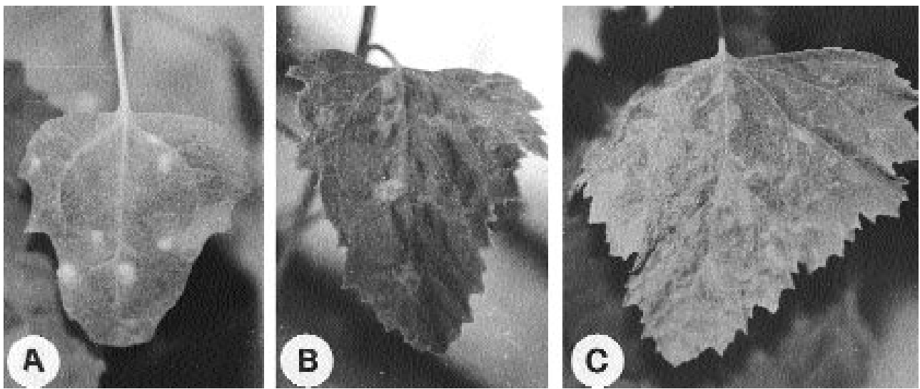
Fig. 1. (A) Chlorotic local lesion on the inoculated leaf of Chenopodium quinoa . Systemic rings (B) and mottling (C) and deformation of the leaves of Chenopodium amaranticolor .
