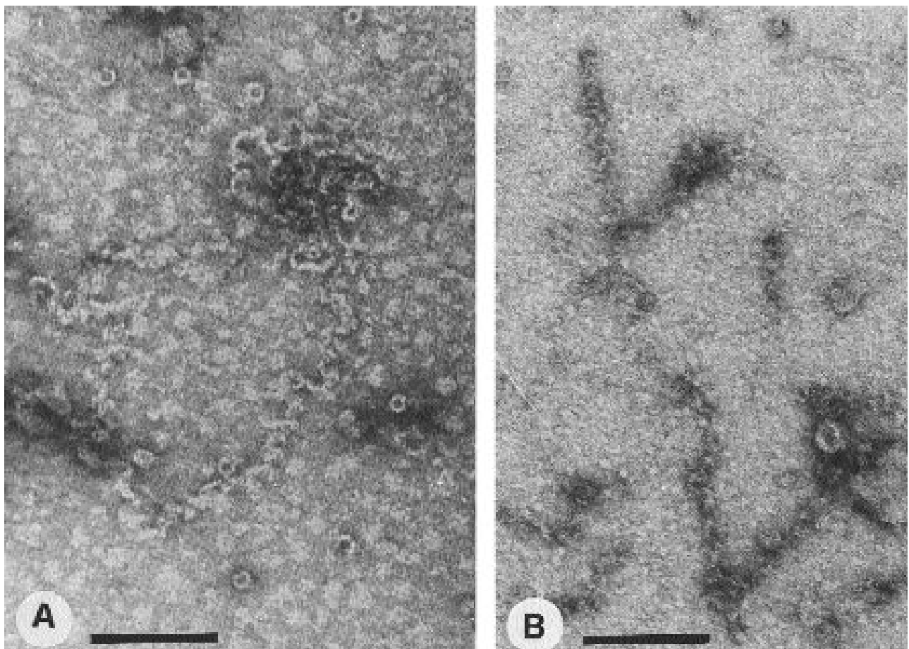
Fig. 2. Negatively stained CPsAV-like particles in the single-stranded open configuration (A) and in the duplex linear form (B) ( sensu Milne et al. , 1996). Bars = 100 nm.
